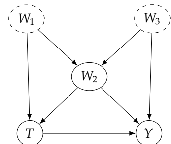
Figure 6.11: Graph where blocking one backdoor path unblocks another
